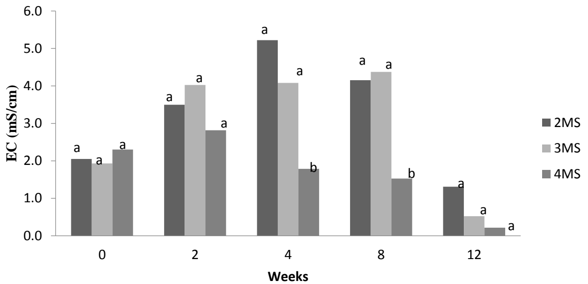
Figure 4.7: Electrical conductivity profile of compost mixed species sawdust
