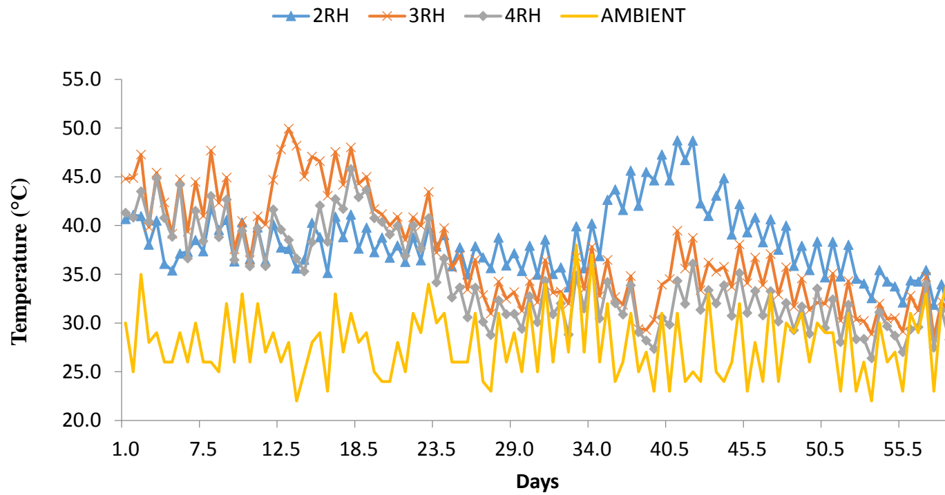
Figure 4.3: Compost temperature as affected by ratio of rice husk to poultry manure
