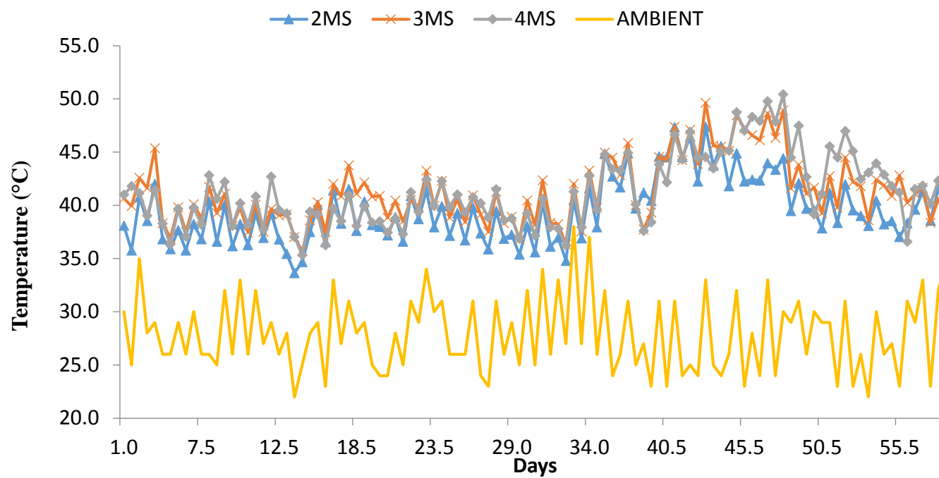
Figure 4.2: Temperature profile of MIXED species sawdust feedstock to poultry manure
