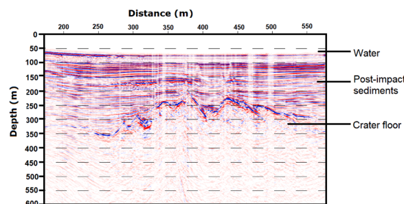
Fig. 6. 2D seismic section across the central uplift of the Bosumtwi impact crater (modified from [48]).
