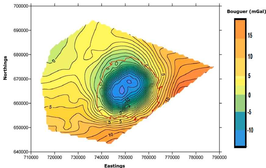
Fig. 7. Lake Bosumtwi preliminary Bouguer anomaly indicating the extent to which rocks are shattered and fractured in the crater area; the solid line marks the lake margin; the rocks in the northern and northwestern area are more affected by the impact (modified after [57]). The map is displayed in the Ghana UTM coordinate system.
