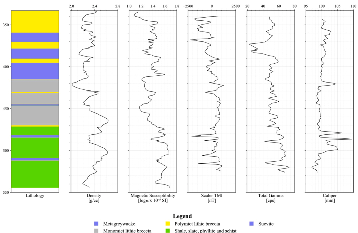
Fig. 8. Physical property logs for borehole LB-07A (data extracted from [43] and replotted).
