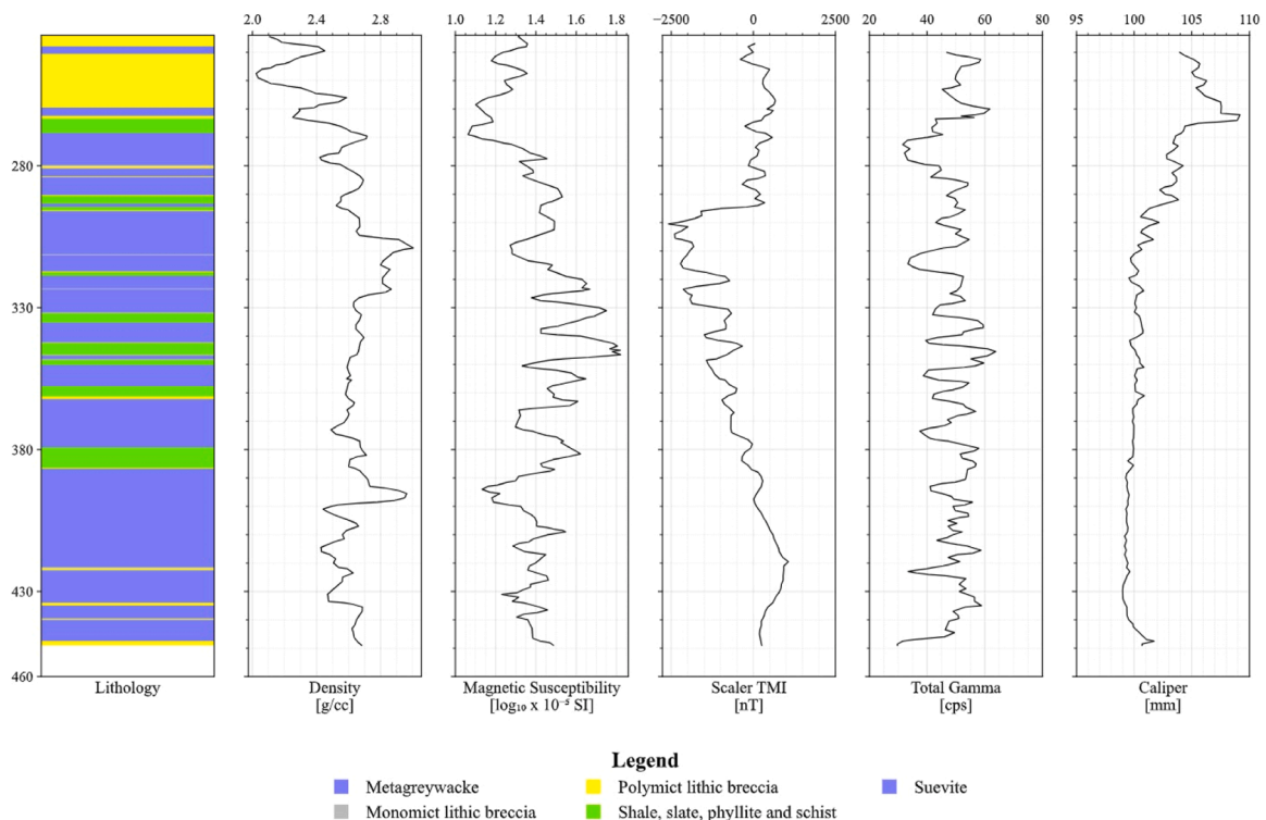
Fig. 9. Physical property logs for borehole LB-08A (data extracted from [43] and replotted).
