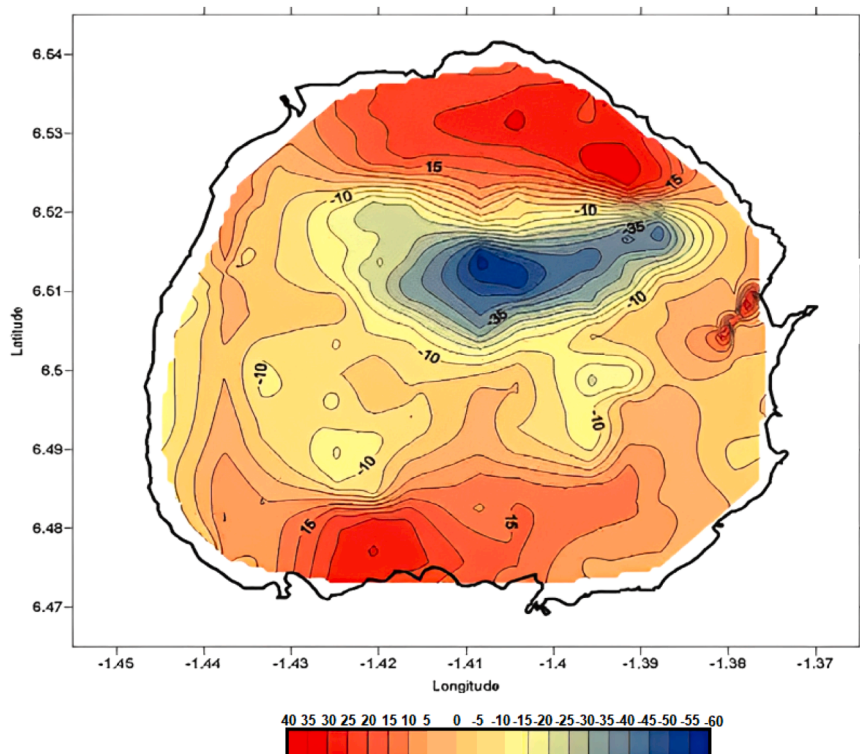
Fig. 5. Magnetic signature of the Bosumtwi impact crater taken across along north-south along the Lake (modified after [57]).
