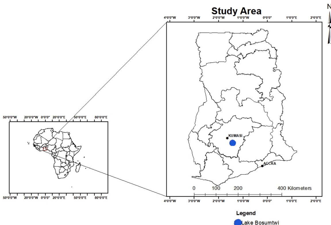
Fig. 2. Location of the Bosumtwi meteorite impact crater in Ghana, West Africa.
