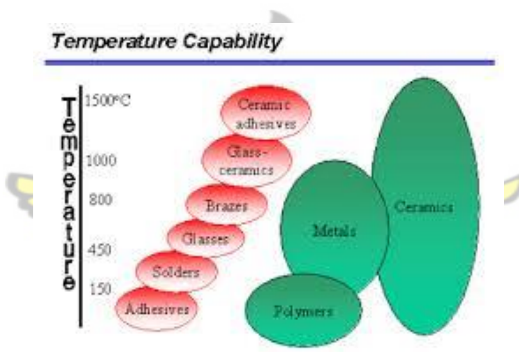
Figure 2.19: Temperature capability of some joining media. Source: Taylor (2016)
