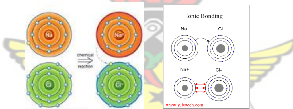
Figure 2.12: Transfer of electrons in ionic bonding Source: www.substech.com
