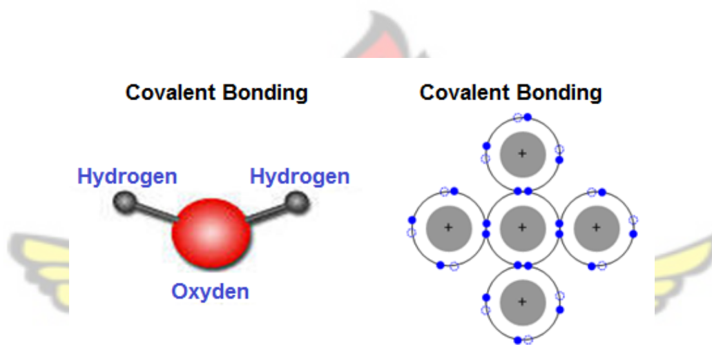
Figure 2.14: Distribution of shells in covalent bonding Source: www.substech.com
