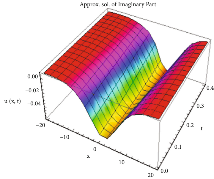
FIGURE 9: NTDM solution of the imaginary part of problem 2.
