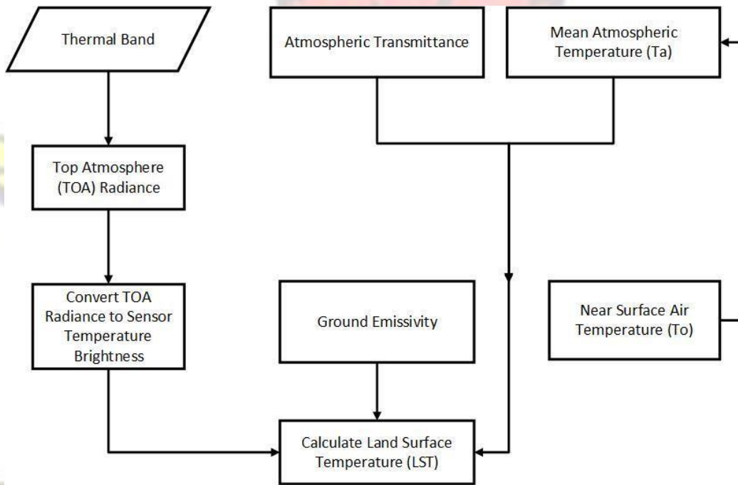
Figure 3-4 Major Steps in Estimating LST
