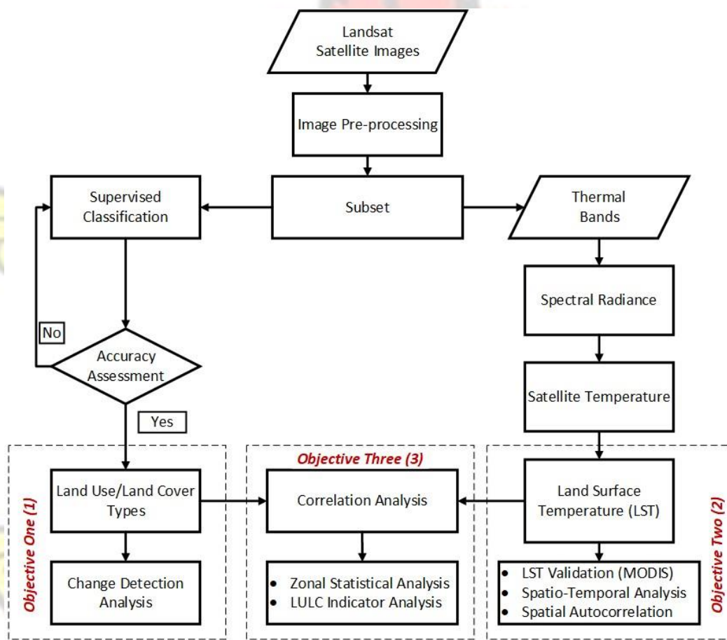
Figure 3-2 Methodology Flowchart
