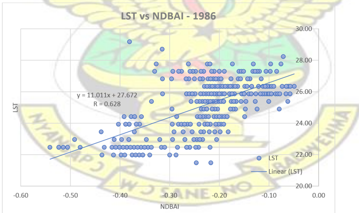
Figure 4-27 Relationship between LST and NDBAI in 1986
