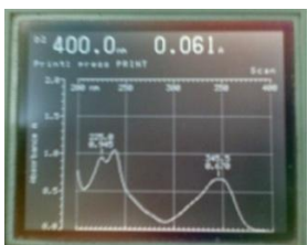
Figure 4.3: 5ml of stock solution diluted to 50ml with 0.1% (v/v) HCl.
