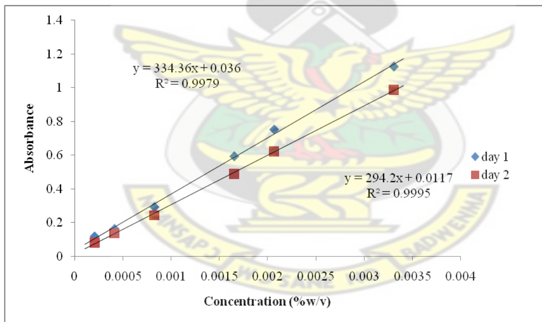
Figure 4.5: Graph of absorbances against concentration of Piperaquine phosphate in 0.001M HCl solution at 349.0nm for two days.
