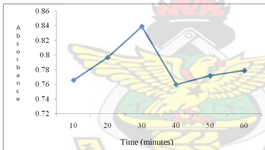
Figure 4.17: 1ml of 1M glacial acetic added to stock solution:
