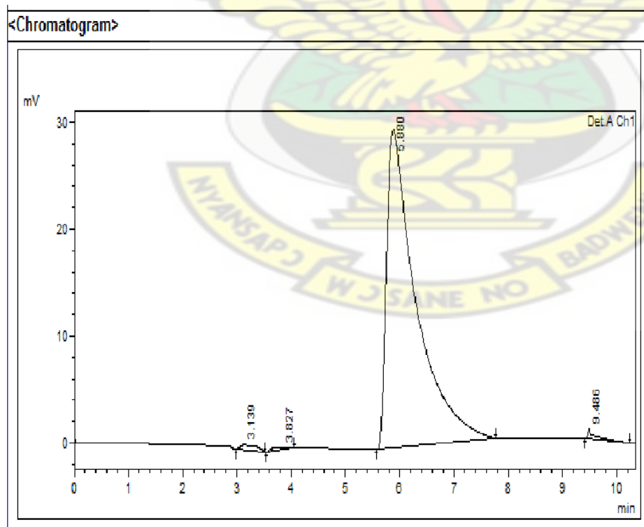
Figure 6.8 Mobile phase- Acetonitrile : Water with 0.1%v/v TFA ( 20: 80)
