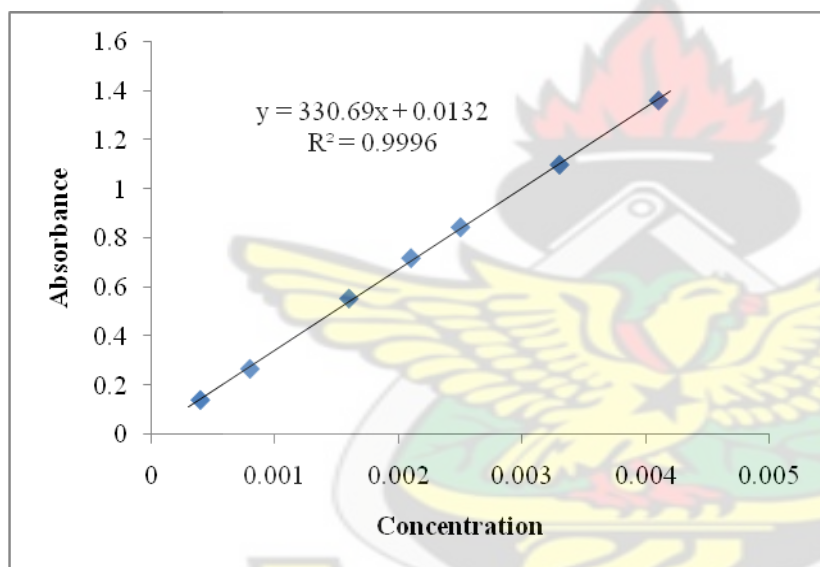
Figure 6.2 UV spectrometry Calibration curves for Piperaquine phosphate (assay of Tablets)
