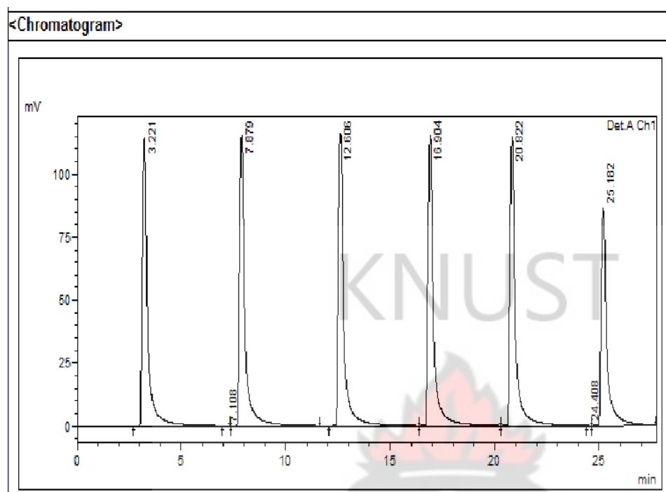
Figure 6.9 Mobile phase- Acetonitrile : Water with 0.1%v/v TFA ( 40: 60)
