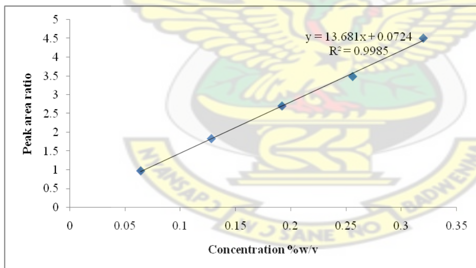
Figure 4.31: Graph of peak area ratio against concentration of DHA
