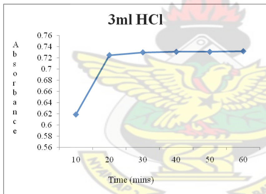
Figure 4.27: Graph of absorbance against time (minutes) of 2ml DHA in MeOH and 3ml HCl
