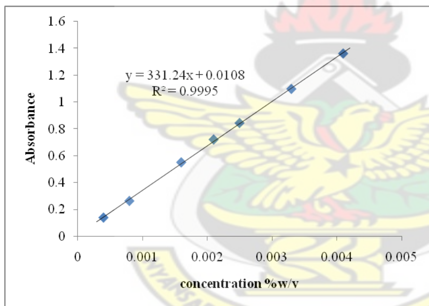
Figure 6.3 UV spectrometry Calibration curves for Piperaquine phosphate (assay of Tablets)
