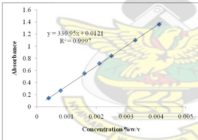
Figure 6.1: UV spectrometry Calibration curves for Piperaquine phosphate (assay of Tablets)
