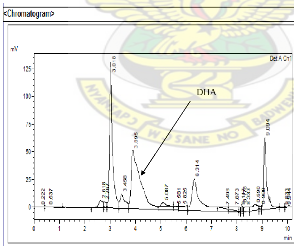
Figure 6.14 Dihydroartemisinin in Tablet B
