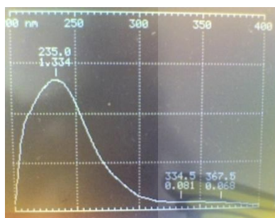
Figure 4.21: 5ml of 0.0253% DHA in MeOH and 2ml 0.7M NH 3 heated at 60°C for 30minutes
