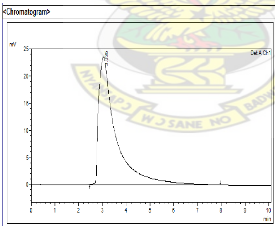
Figure 6.6 Mobile phase- Acetonitrile : Water with 0.1%v/v TFA ( 60: 40)
