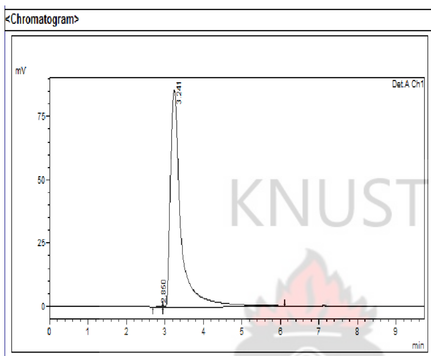
Figure 6.7 Mobile phase- Acetonitrile : Water with 0.1%v/v TFA ( 40: 60)
