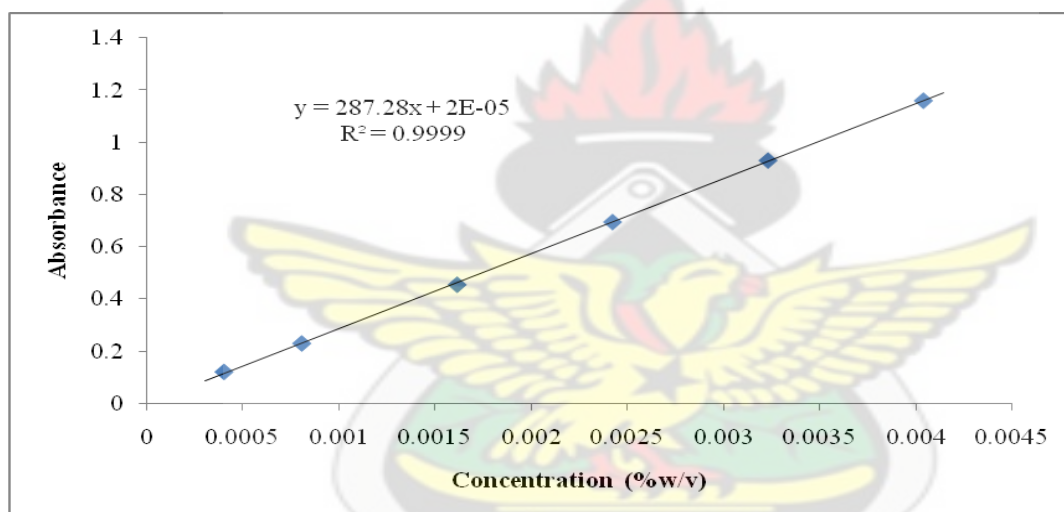
Figure 4.6: Graph of absorbance against concentration of Piperaquine Phosphate in 0.001M HCl solution at 349.0nm.
