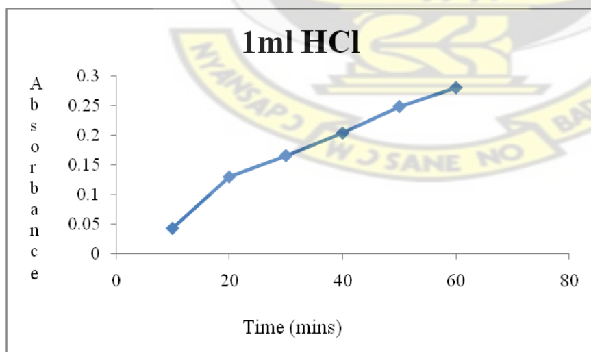
Figure 4.25: Graph of absorbance against time (minutes) of 2ml DHA in MeOH and 1ml HCl
