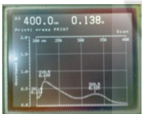
Figure 4.2: 5ml of stock solution diluted to 50ml with 0.05M NaOH.
