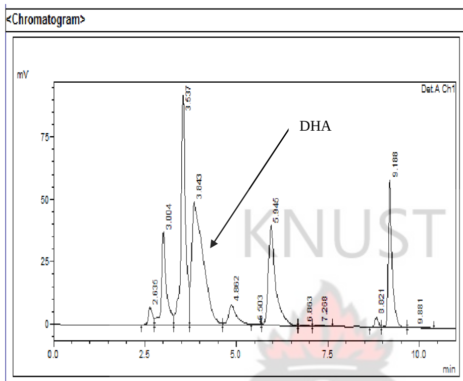
Figure 6.13 Dihydroartemisinin in Tablet A
