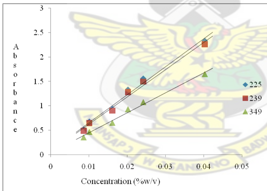
Figure 4.4: Graph of absorbance against concentration of Piperaquine phosphate aqueous solution in 0.001M methanolic HCl at wavelengths of 225.0, 239.0 and 349.0nm
