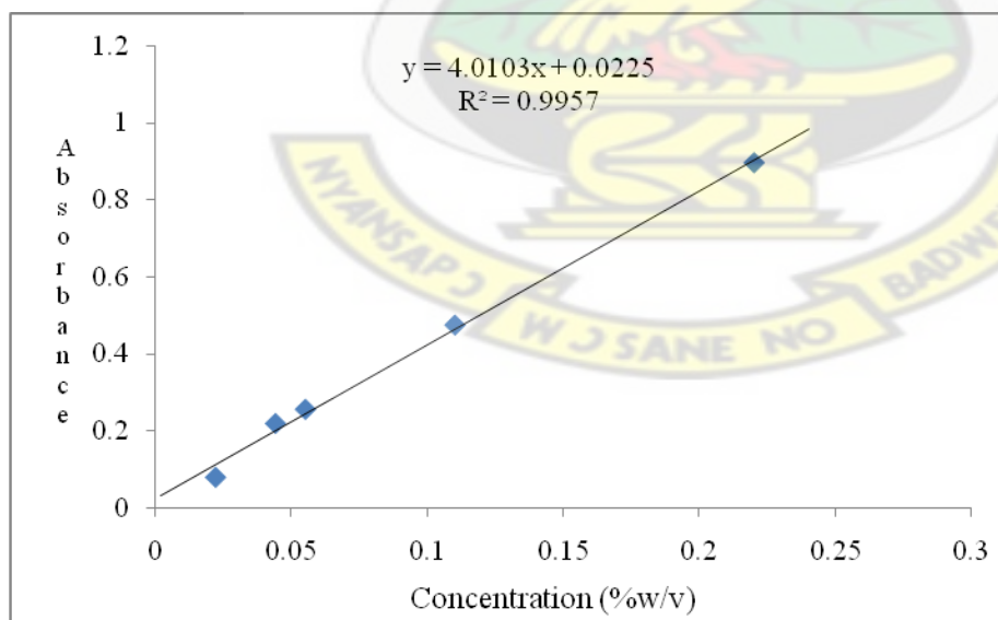
Figure 4.10: A graph of absorbance against concentration of DHA in methanol / 0.05M NaOH heated at 50°C at 289.5nm.
