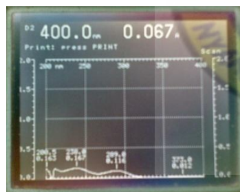
Figure 4.8: 5.00ml of 0.005% (w/v) Dihydroartemisinin in ethanol diluted to 50.00ml with 0.05M NaOH and heated for 30minutes at 50°C
