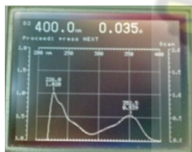
Figure 4.1: 5ml of stock solution diluted to 50ml with water.
