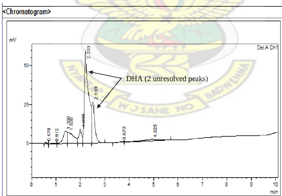
Figure 6.12 Mobile phase- Acetonitrile : Water with 0.1%v/v TFA ( 90: 10)
