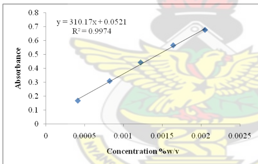
Figure 4.29: Graph of absorbance against concentration of DHA in MeOH/conc HCl solution
