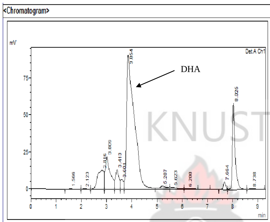
Figure 6.11 Mobile phase- Acetonitrile : Water with 0.1%v/v TFA ( 90: 10)
