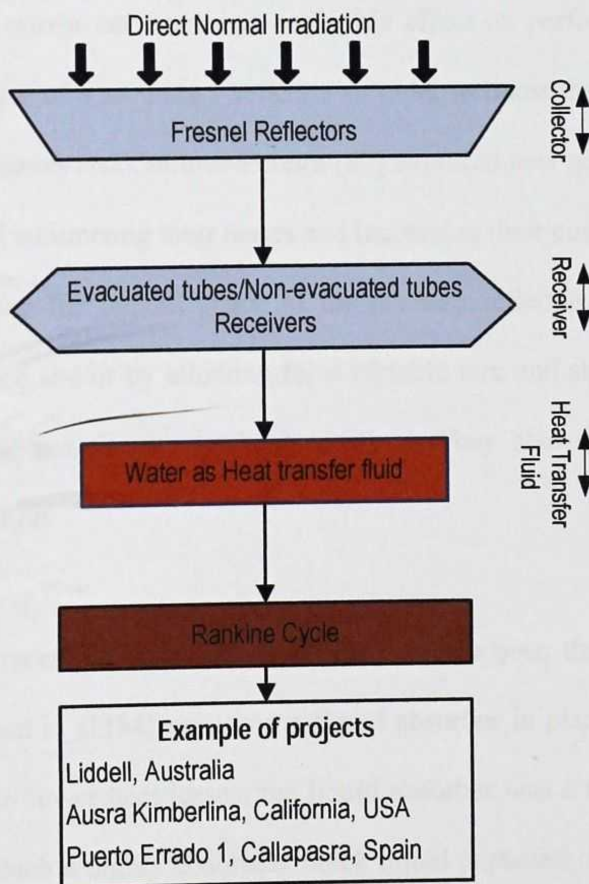
Figure 2.15: Flow chart for Fresnel reflector technology
