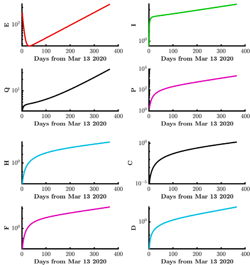
Fig. A.2. One-year simulation dynamics of CoVCom9 model from March 13 2020 when there is a 34% reduction in \phi to \phi = 0.016 . Here E , I , Q , P , H , C , F and D are respectively exposed, infectious, quarantined, confirmed-positive, hospitalised at ordinary ward, hospitalised at intensive care unit, and deaths with the vertical axis on a log-scale. The effect on \mathcal{R}_0 is a change from 3.110 to 2.053.
