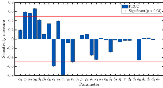
Fig. 5. Sensitivity of the basic reproduction number R_0 to changes in the CoVCom9 parameters using PRCC index.
