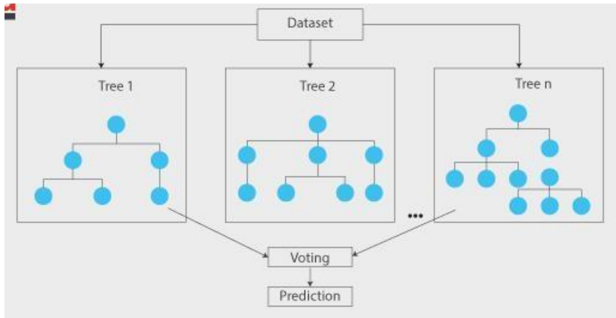
Figure 3-3 Random Forest Model
