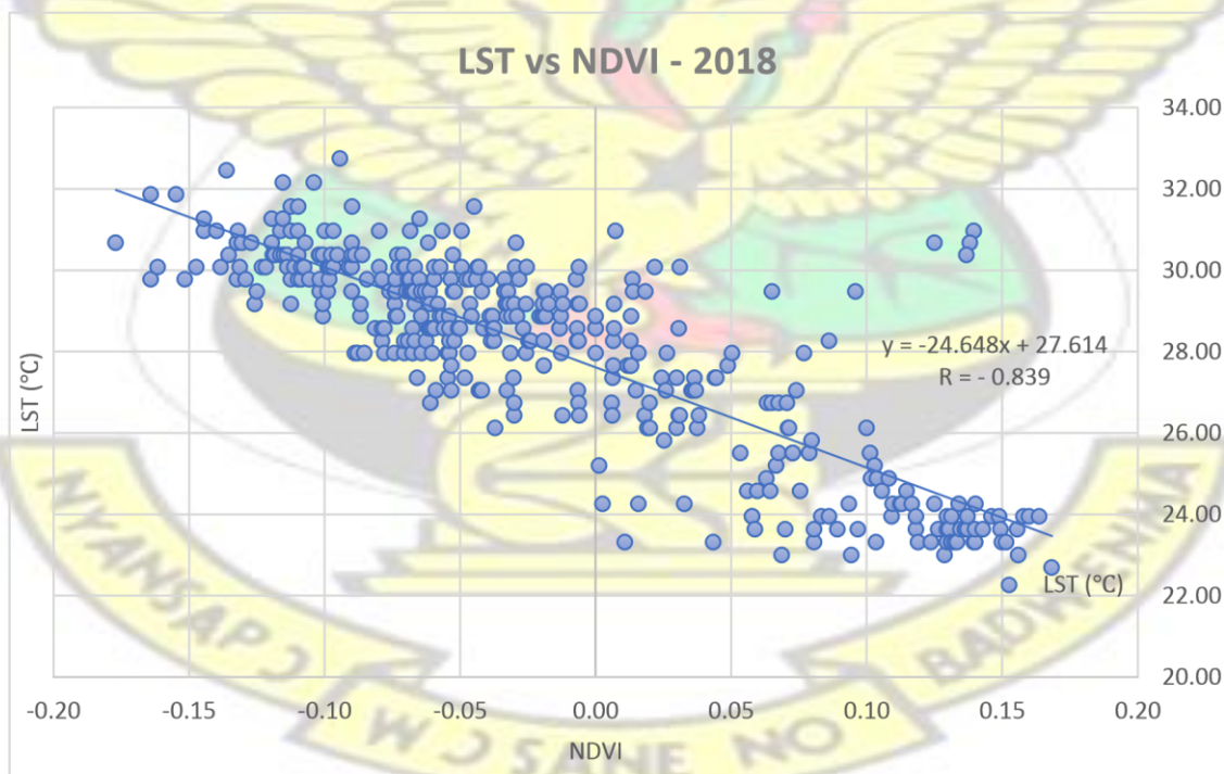
Figure 4-26 Relationship between LST and NDVI in 2018
