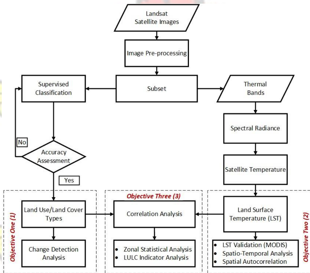
Figure 3-2 Methodology Flowchart
