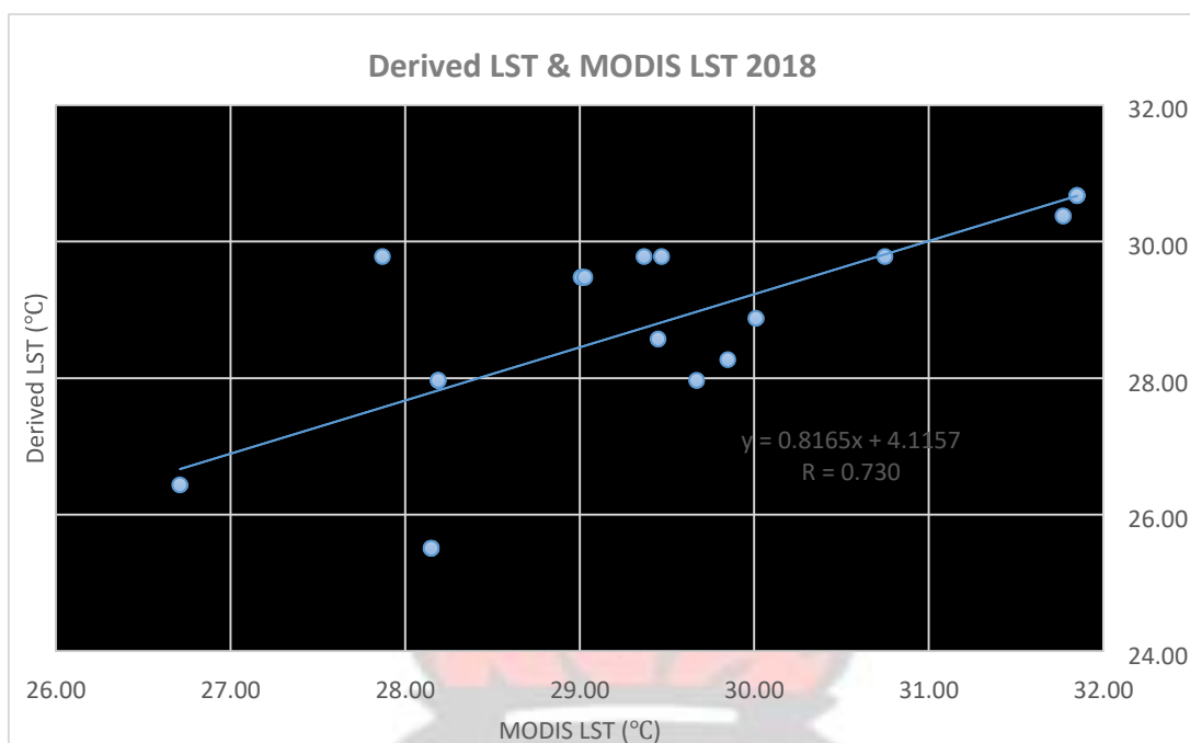
Figure 4-16 Correlation between Derived LST and MODIS LST for 2018
