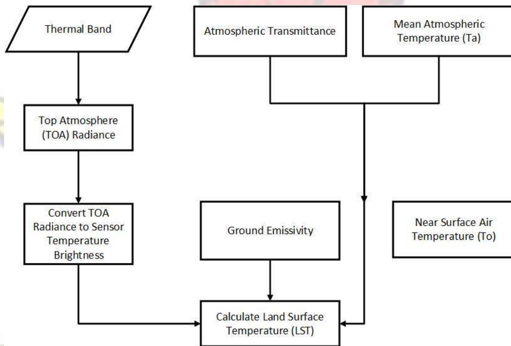
Figure 3-4 Major Steps in Estimating LST
