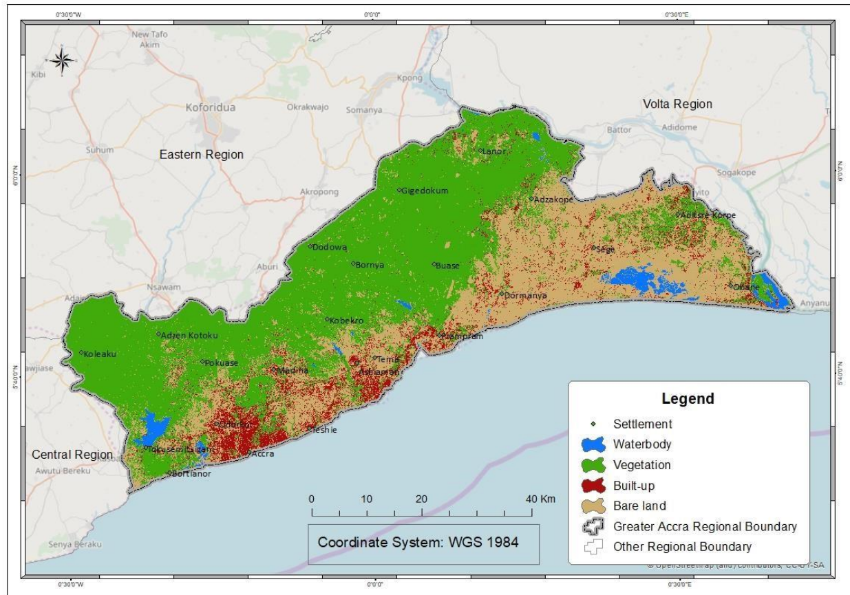
Figure 4-2 LULC Classification Map of 2002
