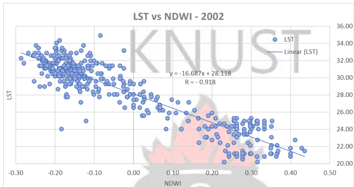
Figure 4-34 Relationship between LST and NDWI in 2002
