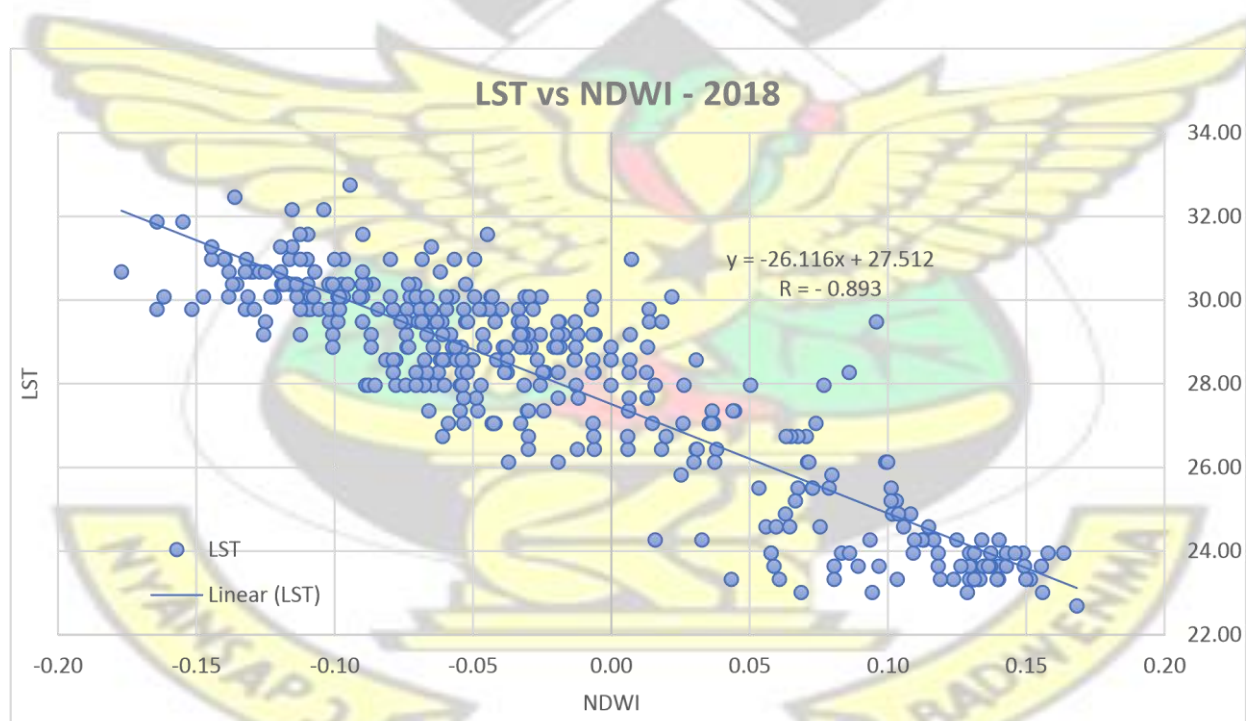
Figure 4-35 Relationship between LST and NDWI in 2018
