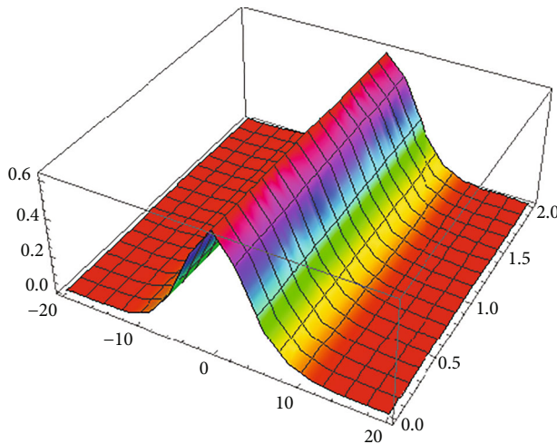
FIGURE 3: 3D surface obtained by exact solution for fractional Kawahara equation at \alpha = 1 .
