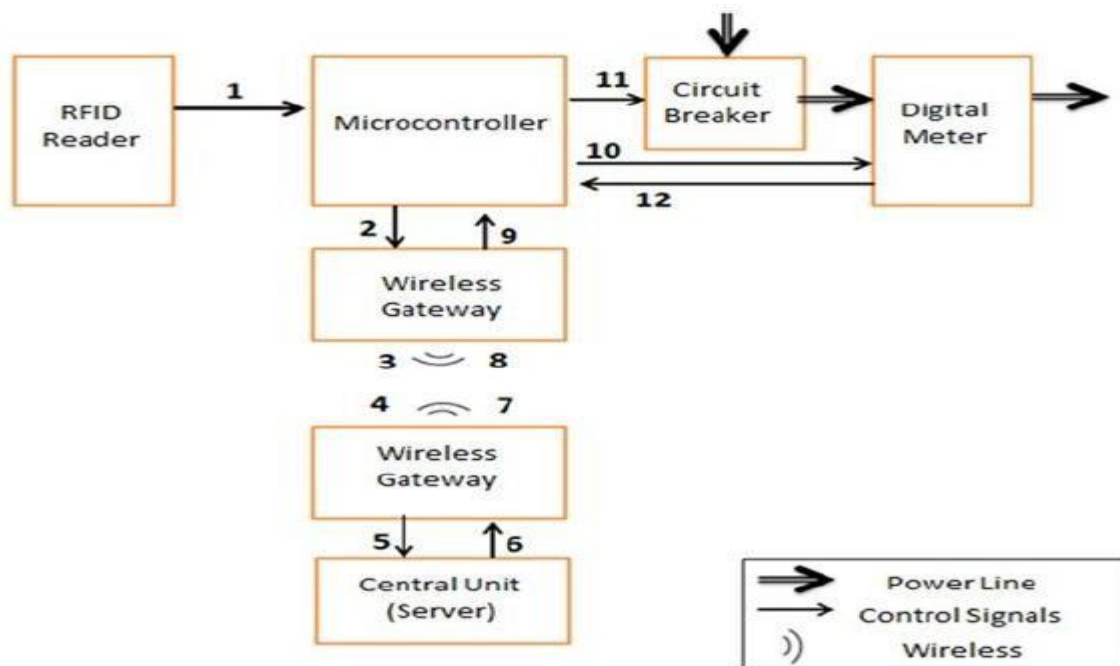
Fig. 2.3 shows the block diagram of the proposed electricity prepaid metering system
