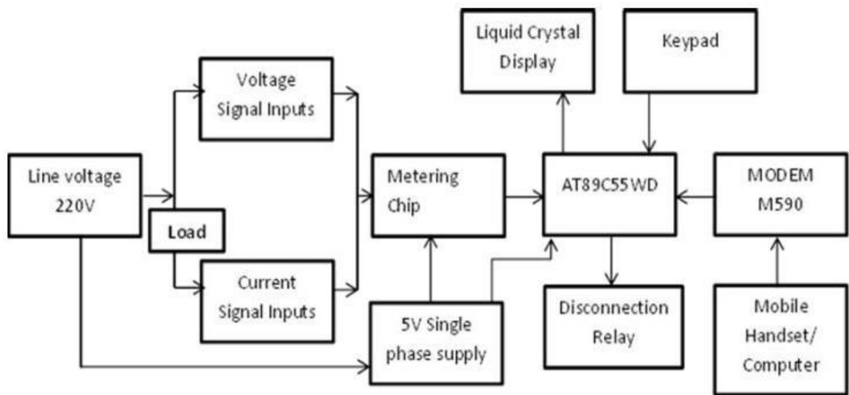
Figure 2.2 : Components of the metering system
