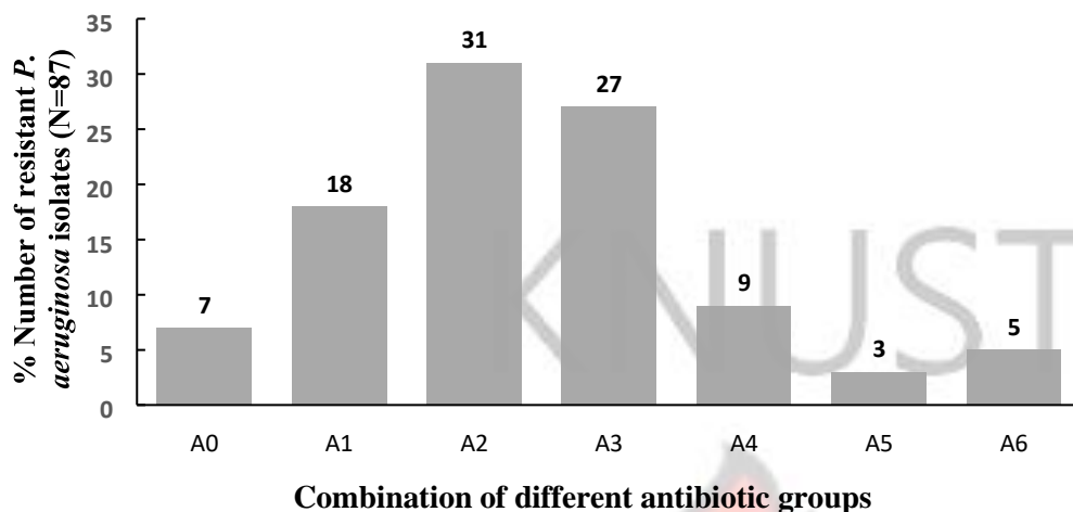
Figure 4.7: Number of resistant P. aeruginosa to the various antipseudomonal groups
