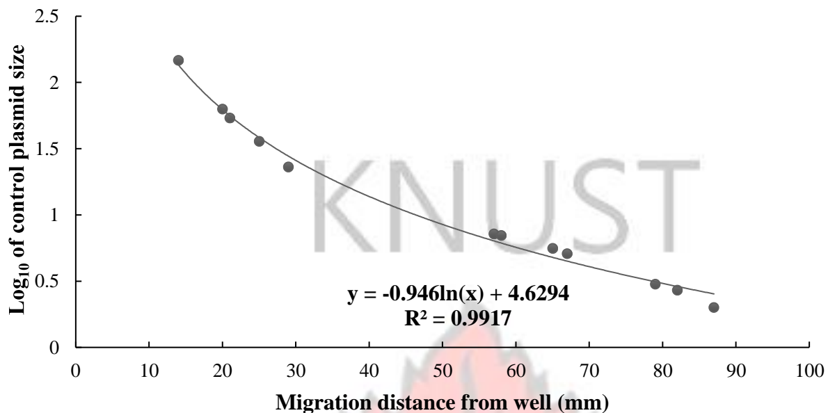
Figure 4.18: Calibration curve for determination of plasmid sizes of P. aeruginosa
