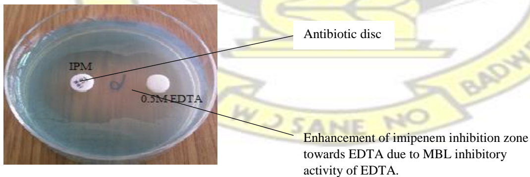
Figure 4.12: Imipenem-EDTA synergy test for detection of metallo- \beta -lactamases production. IPM: Imipenem EDTA: ethylene-diamine-tetraacetic acid.
