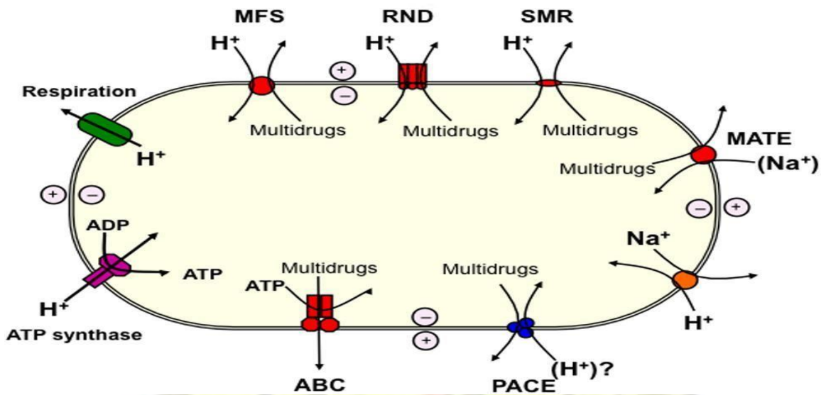
Figure 2.4: Schematic diagram showing multidrug efflux pumps in bacteria and the basis for their energization. Adapted from Hassan et al. , 2015. Major facilitator superfamily (MFS), Resistance nodulation division (RND), Small multidrug resistance (SMR) super families, Multidrug and toxic compound extrusion (MATE) family, ATP-binding cassette (ABC) superfamily, Proteobacterial antimicrobial compound efflux (PACE) family.
