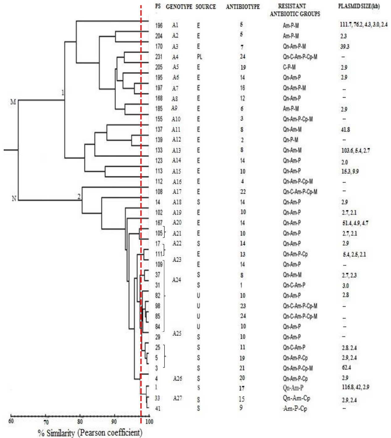
Figure 4.10: Cluster analysis by enterobacterial repetitive intergenic consensus PCR (ERIC-PCR) fingerprinting of 38 multidrug resistant P. aeruginosa isolates generated by Gelj v.1.2 software. S: Stool; U: urine; E: Environment; Qn:quinolone; Am: aminoglycoside; Cp:cephalosporin; C:carbapenem; P:penicillin; M: Cluster I; N : Cluster II.
