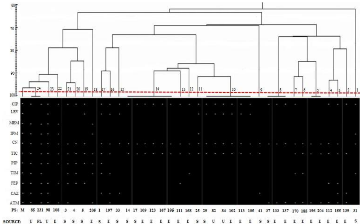
Figure 4.8: Dendrogram derived from antibiogram using Gelj ver.1.2 with Dice coefficient and UPGMA (unweighted pair group method with arithmetic averages). PS 1-231: Pseudomonas aeruginosa isolate, U: Urine; S: Stool; E: Environment; PL: Poultry litter; M: resistance marker
