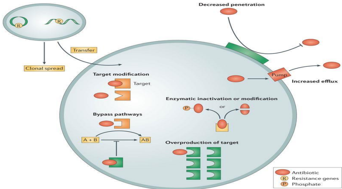
Figure 2.3: Mechanism of antibiotic resistance in bacteria (Adapted from Lewis, 2013)
