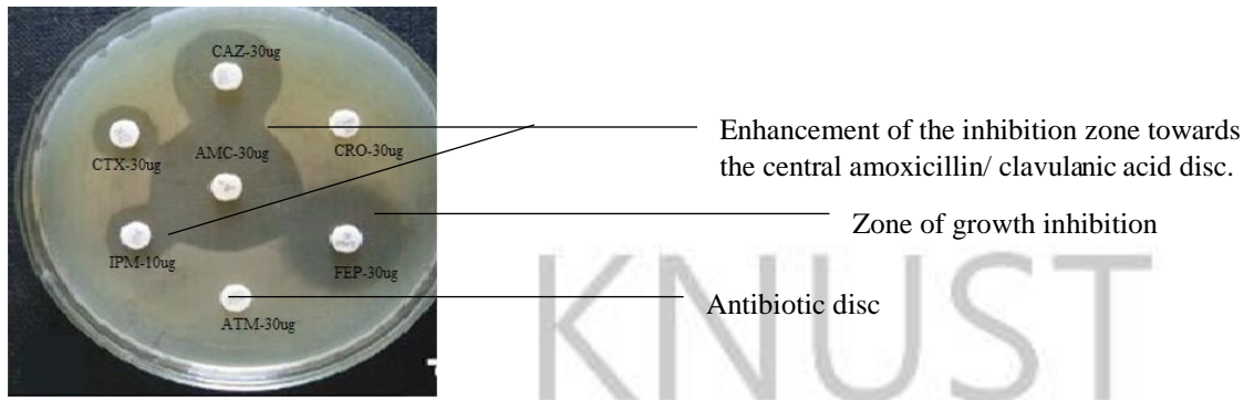
Figure 4.11: Double disk synergy test (DDST) showing production of extended spectrum beta-lactamase (ESBL) in MDR P. aeruginosa . AMC-30 µg: Amoxicillin/clavulanic acid 30 µg; CAZ-30 µg: Ceftazidime 30 µg; CRO-30 µg: Ceftriaxone 30 µg; FEP-30 µg: Cefepime 30 µg; ATM-30 µg: Aztreonam 30 µg; IPM-10 µg: Imipenem 10 µg; CTX-30 µg: Cefotaxime.
