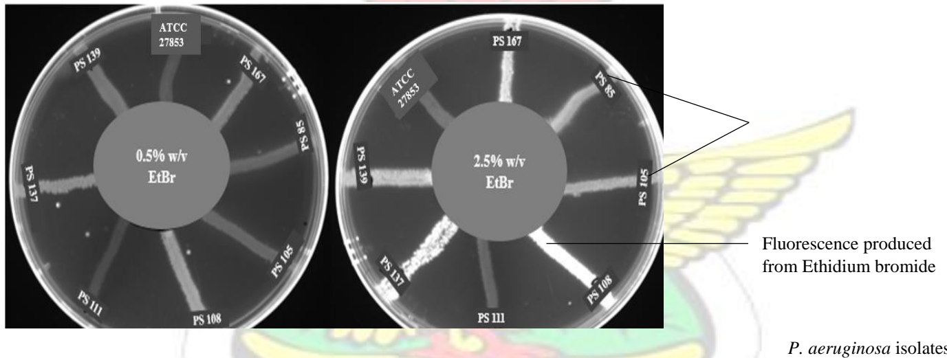
Figure 4.14: Fluorescence of MDR P. aeruginosa on Ethidium bromide incorporated Mueller-Hinton agar plates. EtBr: Ethidium bromide
