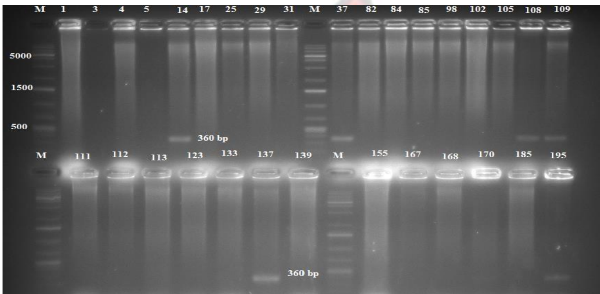
Figure 4.15: Gel image showing amplification of a 360 bp gyrA gene in MDR P. aeruginosa . M: molecular; 1- 195: P. aeruginosa isolates.
