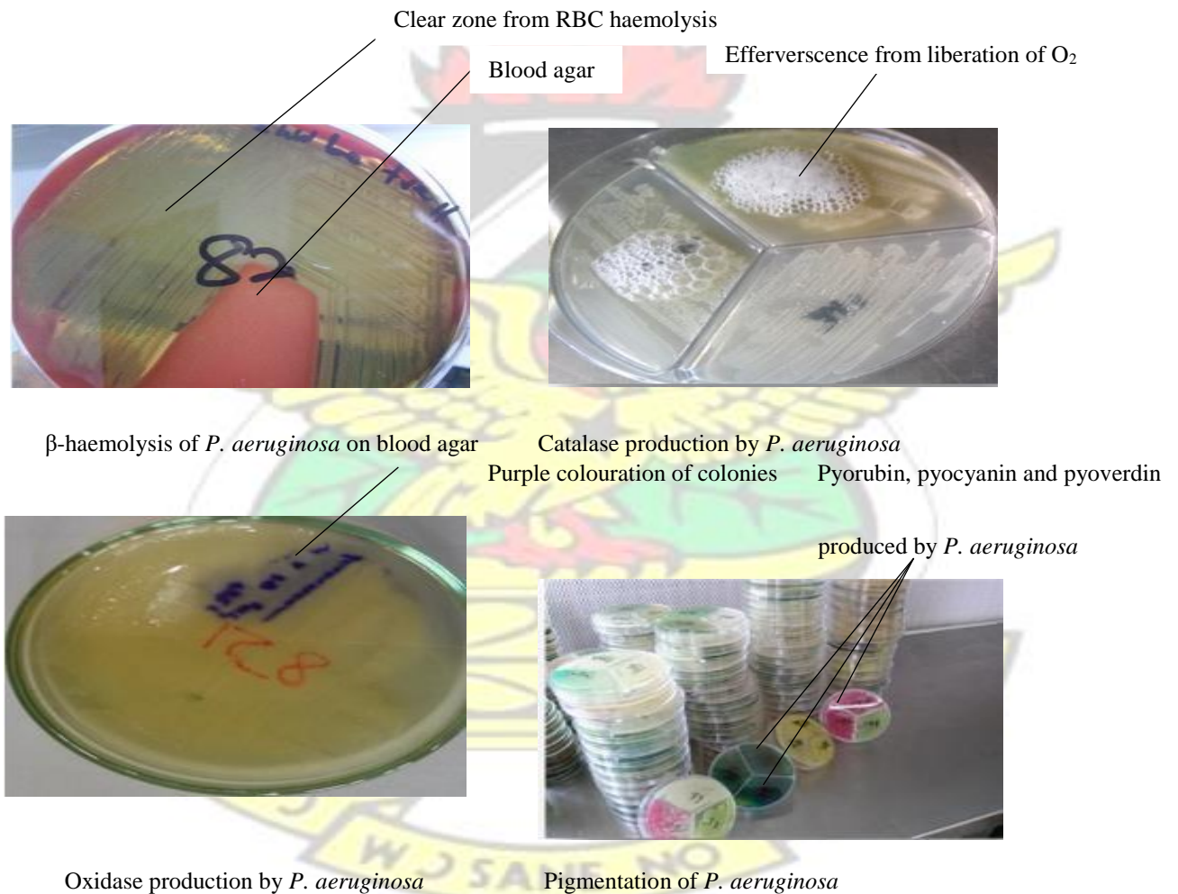
Figure 4.1a: Biochemical characteristics of clinical, environmental and poultry litter P. aeruginosa isolates.
