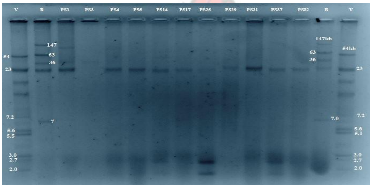
Figure 4.17: Image of a gel showing number and sizes of plasmids in MDR P. aeruginosa isolates. V 517= E. coli control strain V517; R 39 = E. coli control strain R39; C-DNA-Chromosomal DNA
