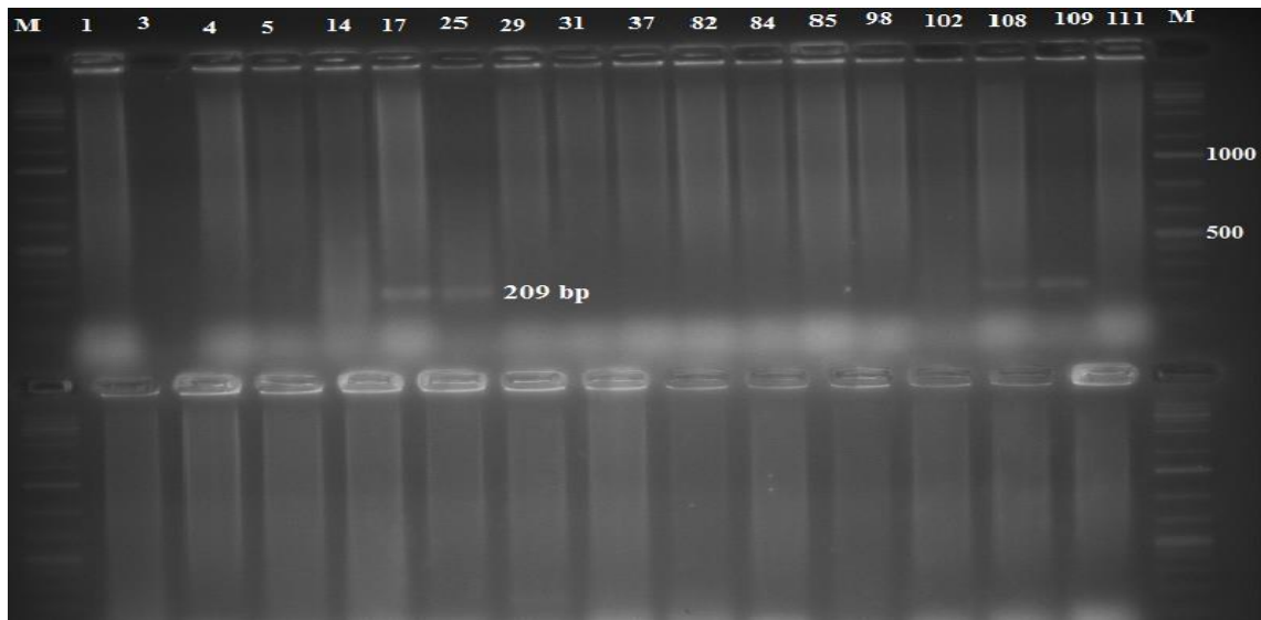
Figure 4.16: Gel image showing 209 bp amplified parC gene in P. aeruginosa .
