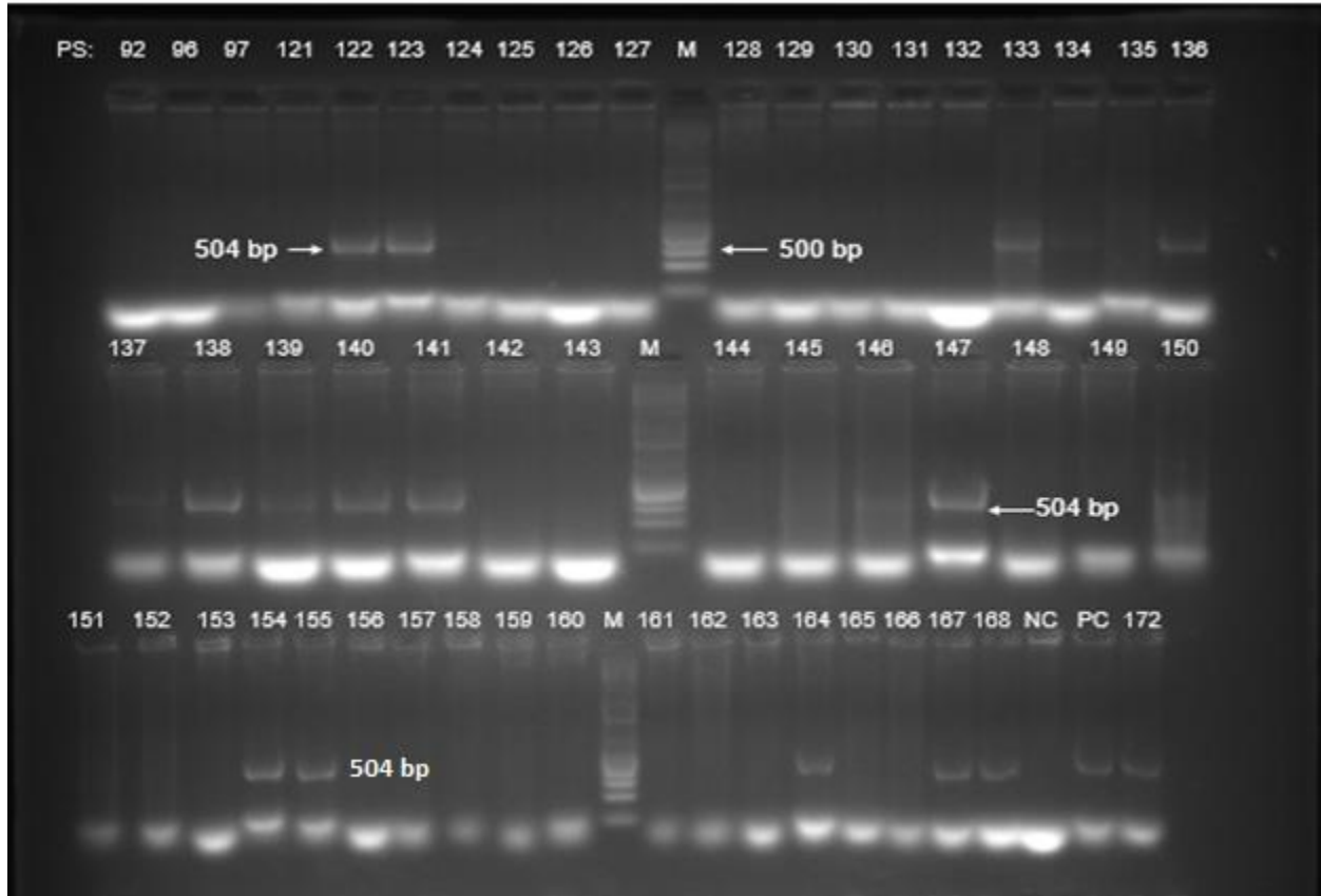
Figure 4.2: Gel image showing a 504 bp PCR amplicon of a peptidoglycan associated outer membrane lipoprotein gene ( oprL ) in P. aeruginosa . M: DNA marker; PC: positive control ( Pseudomonas aeruginosa ATCC 27853); NC: Negative control
