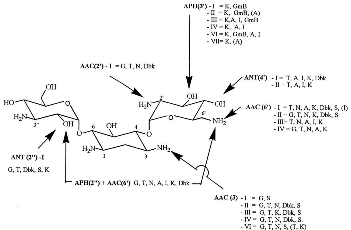
Figure 2.5: Sites of action and antibiotic substrate specificities of aminoglycoside modifying enzymes. A, amikacin; Dbk, dibekacin; G, gentamicin; I, isepamicin; Km, kanamycin; Lv, lividomycin; N, netilmicin; S, sisomicin; T, tobramycin. (Available at www.lookfordiagnosis.com/mesh_info.php?term=aminoglycosides&lang=1 ). Accessed March 2016
