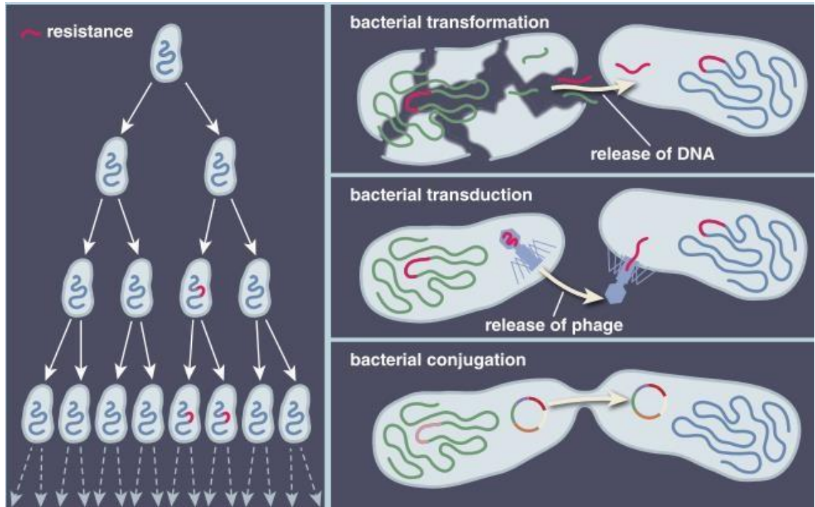
Figure 2.2: Horizontal and vertical transfer of resistance genes in bacteria (Adapted from Dantas and Sommer, 2014)
