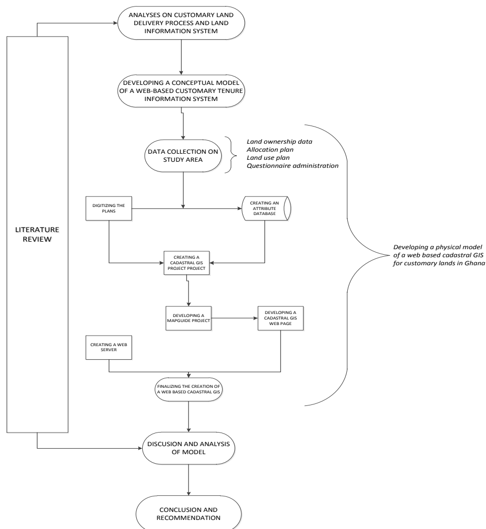
Fig. 1.2: Research methodology.
