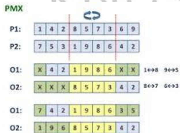
Figure 3.6: Partially Matched Crossover
