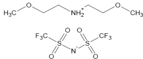
2 bis(2-methoxyethyl)ammonium bis(trifluoromethylsulfonyl)imide
