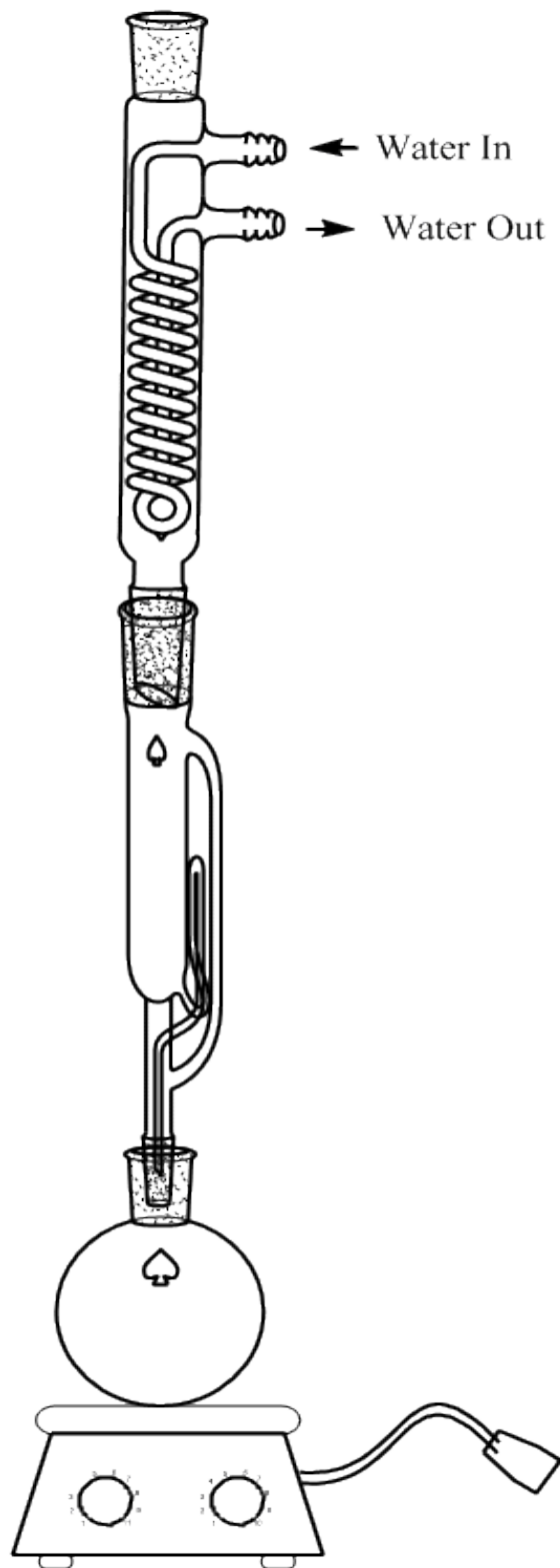
Plate 3.2: Experiment Setup for Batch Percolation
