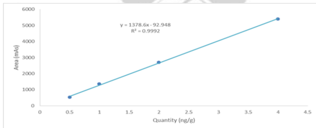
Figure 3.2 Calibration curve of OTA
