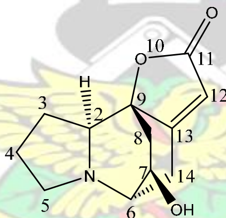
Figure 5.5.1.6: 3D structure of compound Pf6 (epibubbialine)
