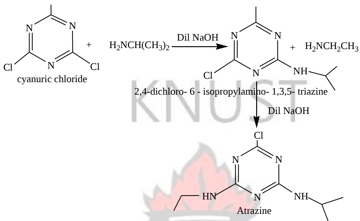
Scheme 1: Synthetic pathway of atrazine.
