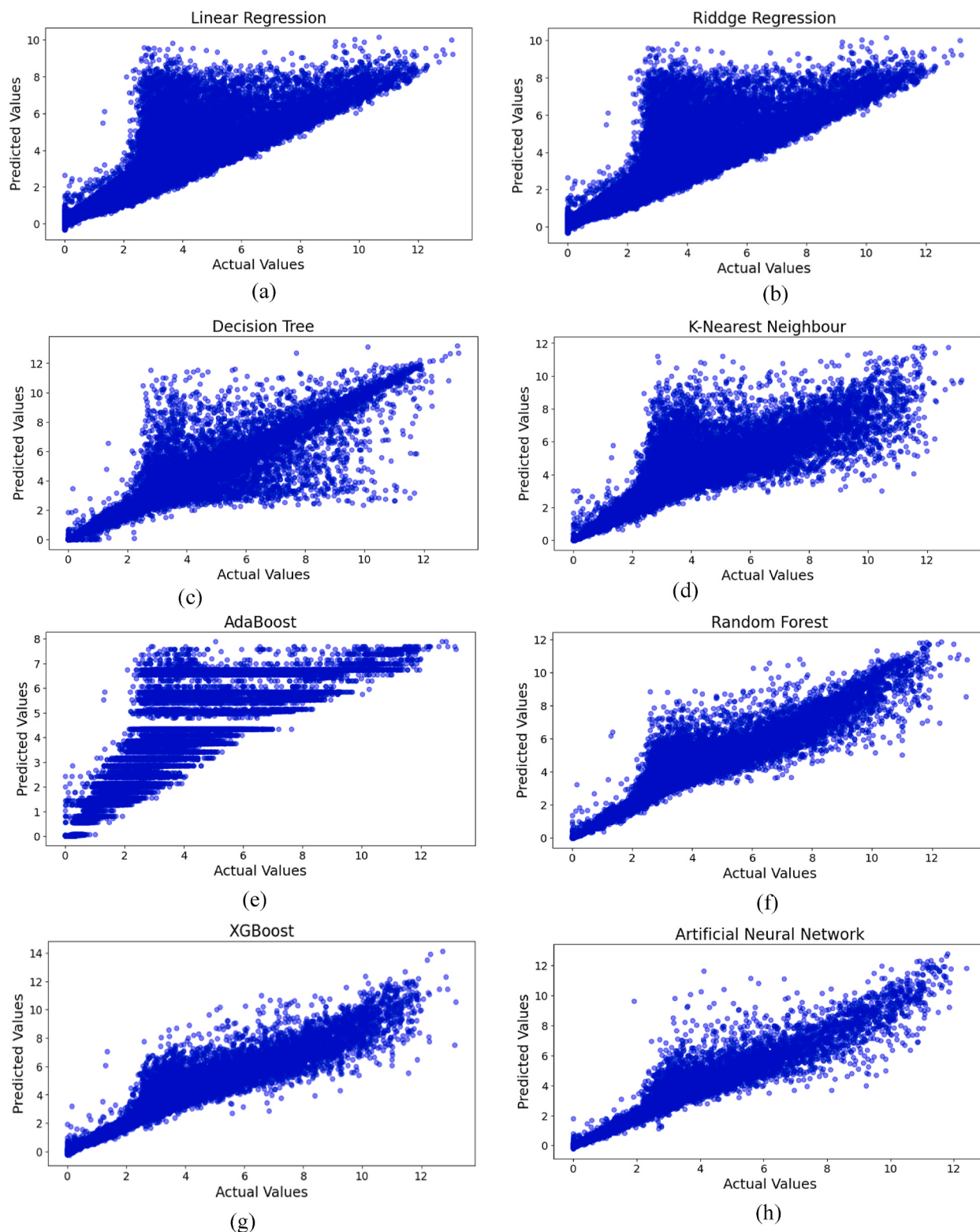
Fig. 8. Regression plot of predicted and actual values using (a) Linear Regression (b) Ridge Regression (c) Decision Tree (d) K-Nearest Neighbour (e) AdaBoost (f) Random Forest (g) XGBoost and (h) Artificial Neural Network.
