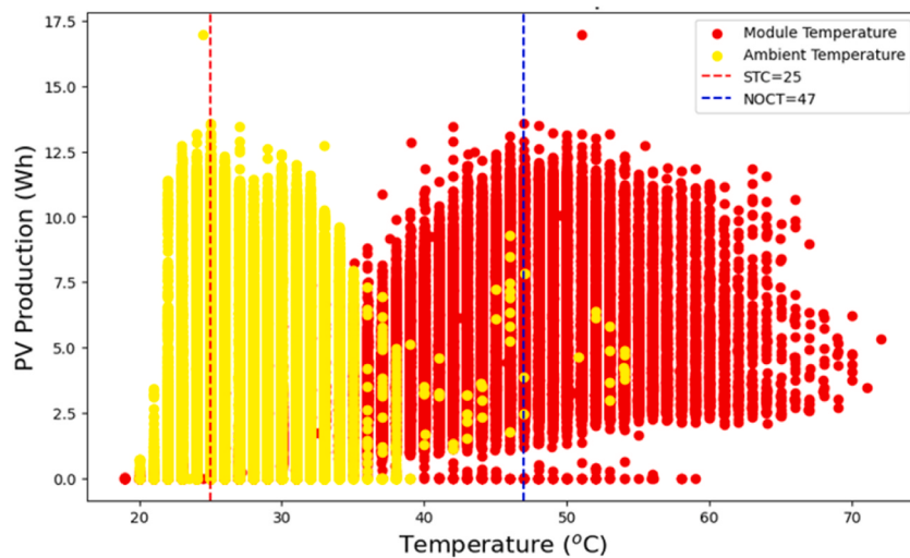
Fig. 7. Effect of Temperature on solar PV output.
