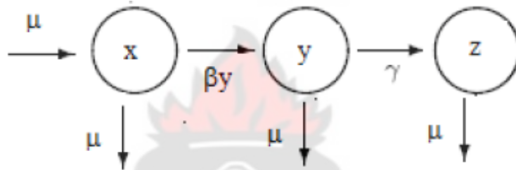
Figure 2.1: A Compartmental model for Measles
