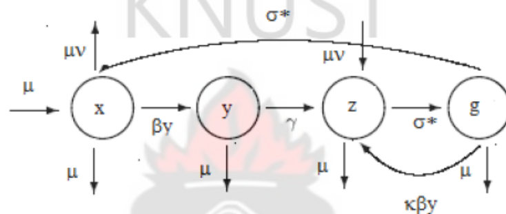
Figure 2.2: A Compartmental model for Whooping cough
