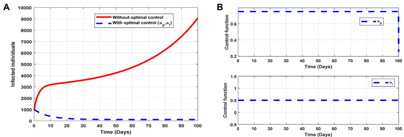
FIGURE 10 Optimal solutions of implementing strategy 5. Plot (A) blue dotted line is the optimal solution for implementing strategy 5. (B) Optimal control profiles for strategy 5.
