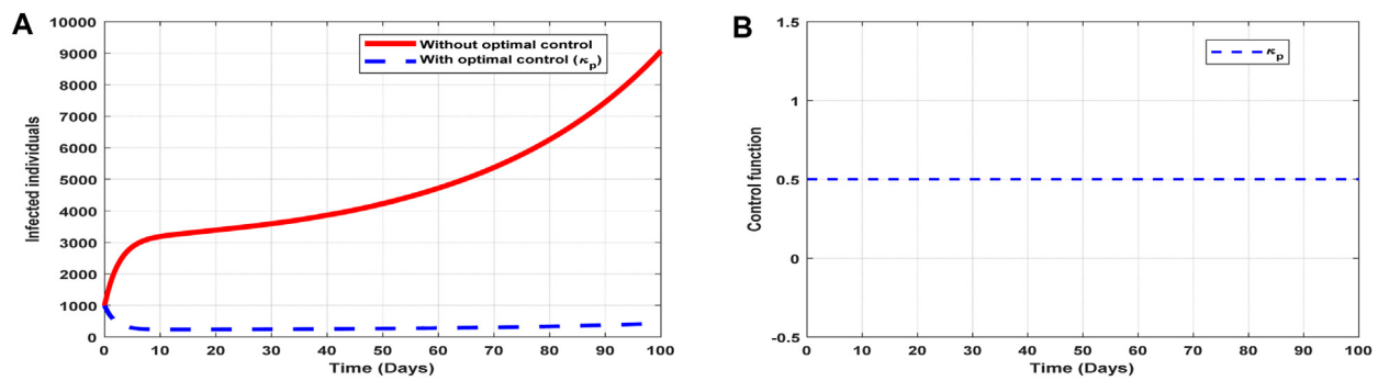
FIGURE 6 Optimal solutions of implementing strategy 1. Plot (A) blue dotted line is the optimal solution for implementing strategy 1. (B) Optimal control profile for strategy 1.
