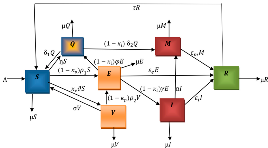
FIGURE 1 SVEQIMR model flowchart.
