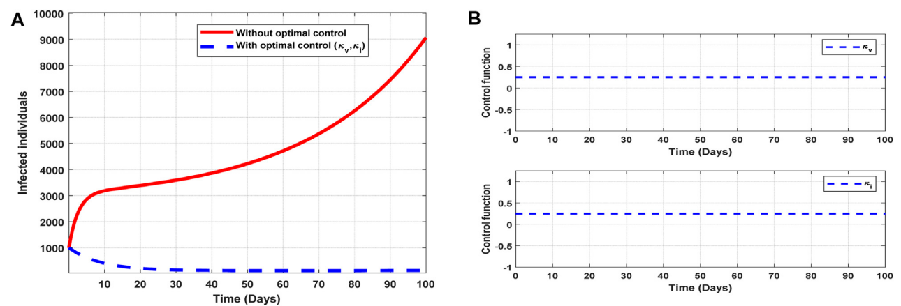
FIGURE 11 Optimal solutions of implementing strategy 6. Plot (A) blue dotted line is the optimal solution for implementing strategy 6. (B) Optimal control profiles for strategy 6.
