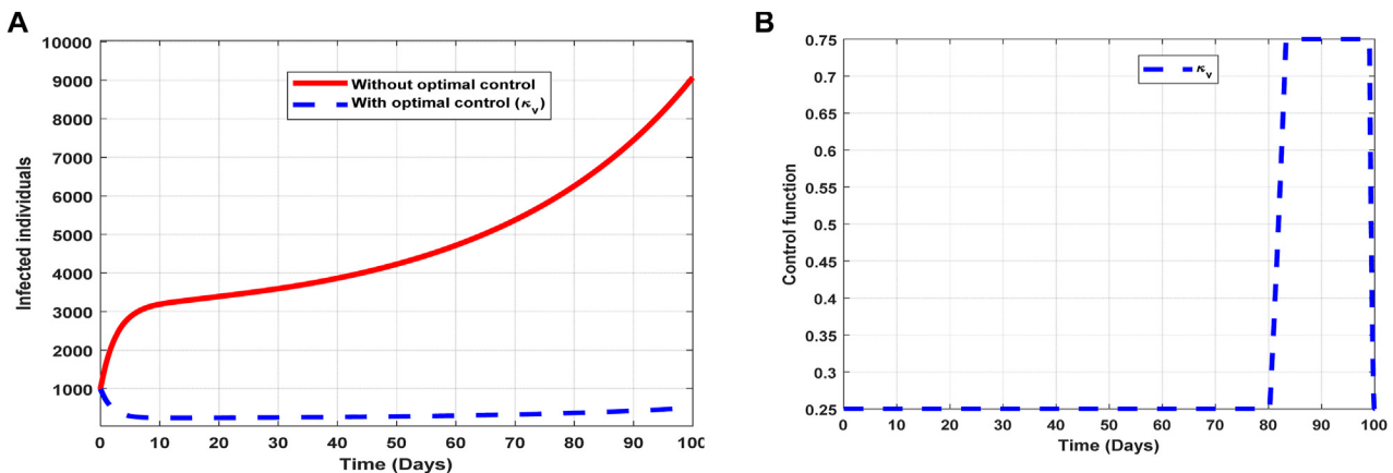
FIGURE 7 Optimal solutions of implementing strategy 2. Plot (A) blue dotted line is the optimal solution for implementing strategy 2. (B) Optimal control profile for strategy 2.
