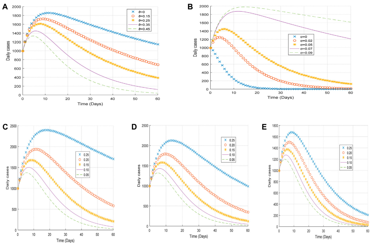
FIGURE 5 Plot of (A) the impact of vaccination rate \theta on COVID-19 daily cases (B) and the impact of vaccine inefficacy \sigma , (C) infectivity reduction of exposed individuals r_e , (D) infectivity reduction of quarantined individuals r_q , and (E) infectivity reduction of isolated individuals r_m on COVID-19 daily cases.
