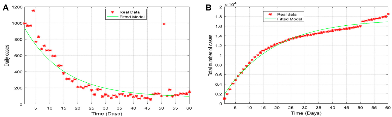
FIGURE 4 Plot of (A) the daily cases and (B) the total number of cases of the fitted model versus the real data from 1st January to 1st March 2022.
