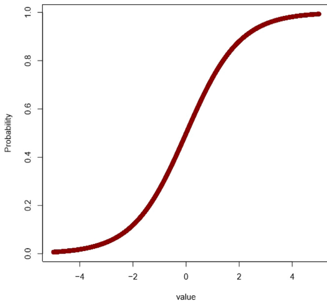
Fig. 4. Logistic curve.
