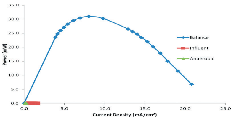
Figure 1. Power density curve for three different wastewaters from same source, but three different treatment methods.
